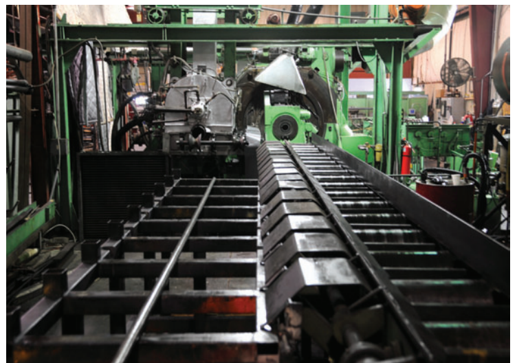
Radial forge runout table
